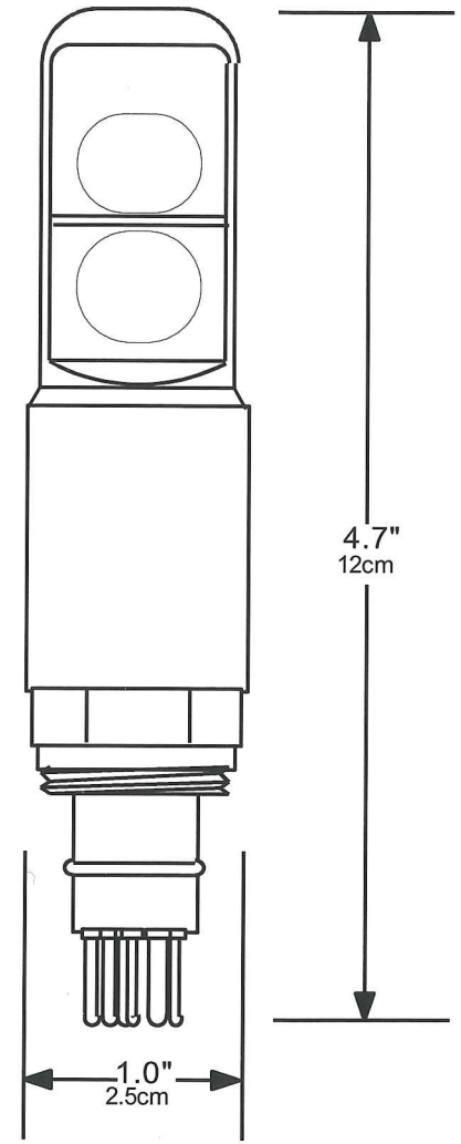
Figure 1. Outline Drawing
