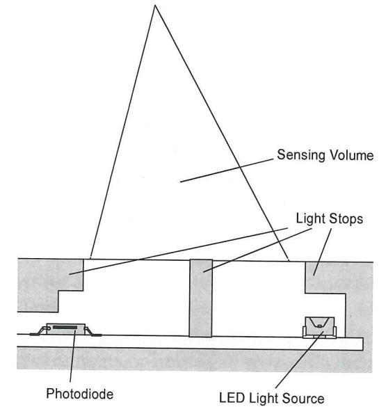
Figure 2. Diagram of Seapoint Turbidity Meter Optics
