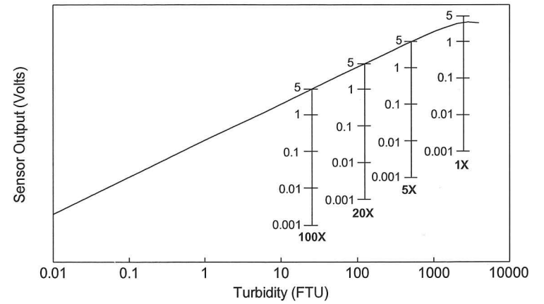
Figure 4. Sensor Response to Formazin Turbidity Standard
